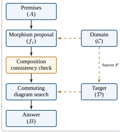
Figure 1. AAAI-style schematic of the CAI inference path. Transformer proposals are filtered through categorical constraints: morphism chains must compose lawfully, cross-domain transfer is mediated by functors, and alternative routes are compared through approximate diagram commutativity.
